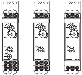
H3DK-M2 H3DK-S2
