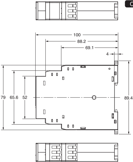
H3DK-S1
